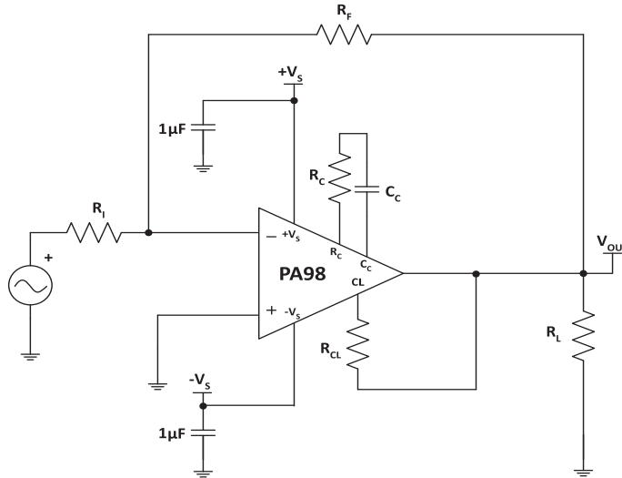
Figure 2: Typical Connections
