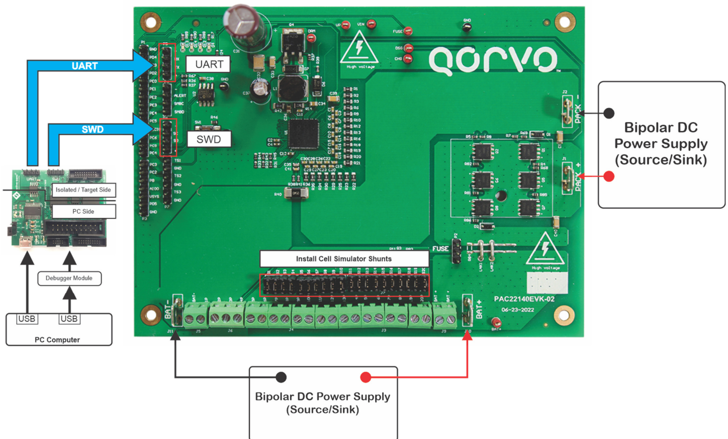
Figure 6: PAC22140EVK with Dual Sink Source Supply Evaluation
