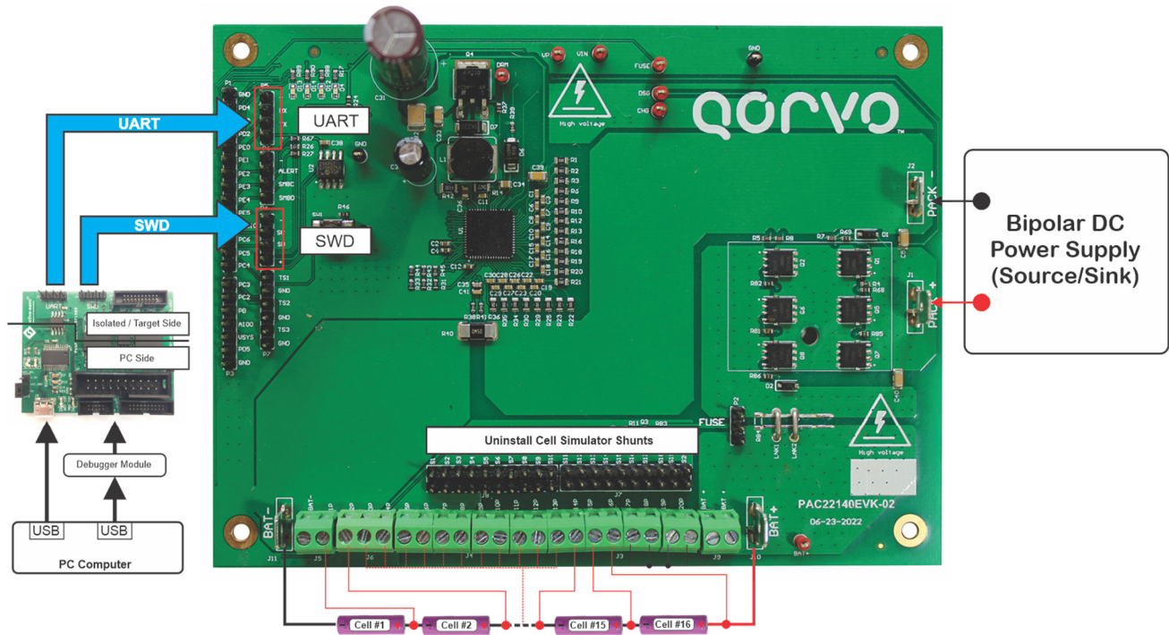
Figure 7: Evaluate PAC22140EVK with Cells Stack
