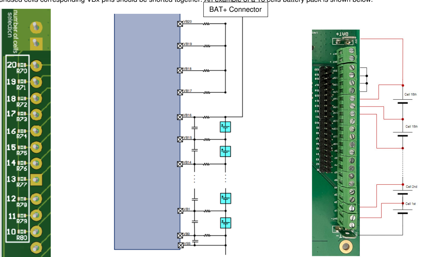
Figure 4: Cell Count Connection guide
