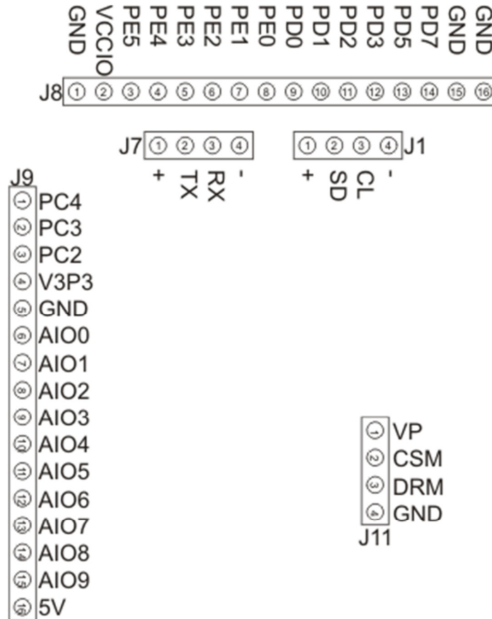
Figure 2 PAC5222EVK1 Headers and Test Stakes Pinout
