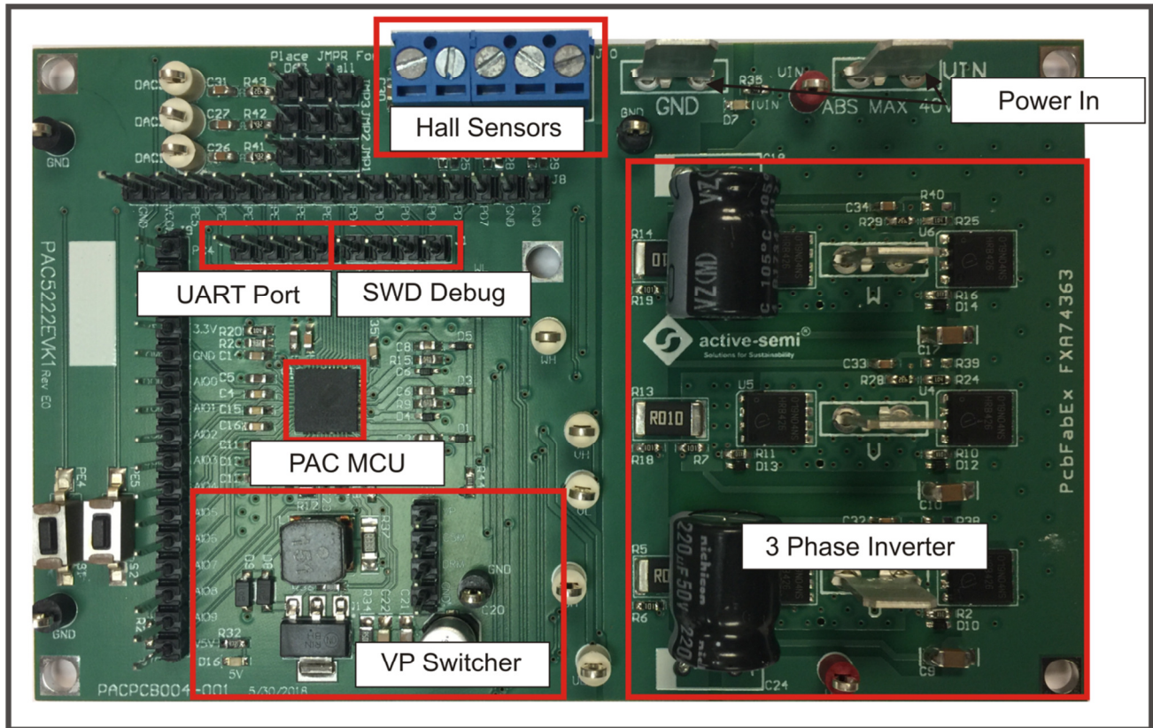
Figure 1: PAC5222EVK1 Block Diagram
