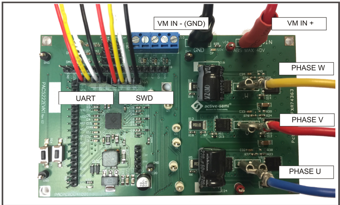
Figure 4: PAC5222EVK1 Evaluation Module Connections
