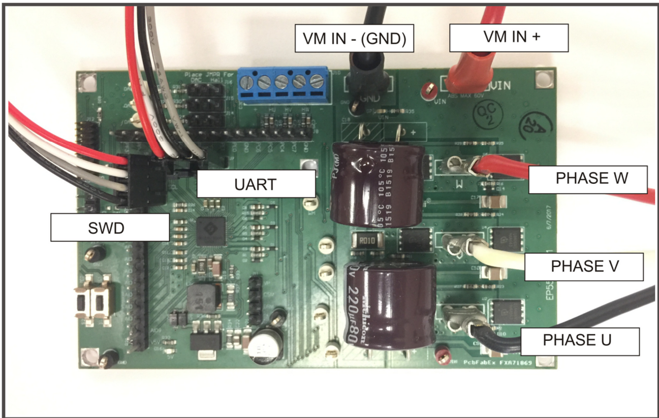
Figure 4: PAC5523EVK1 Evaluation Module Connections
