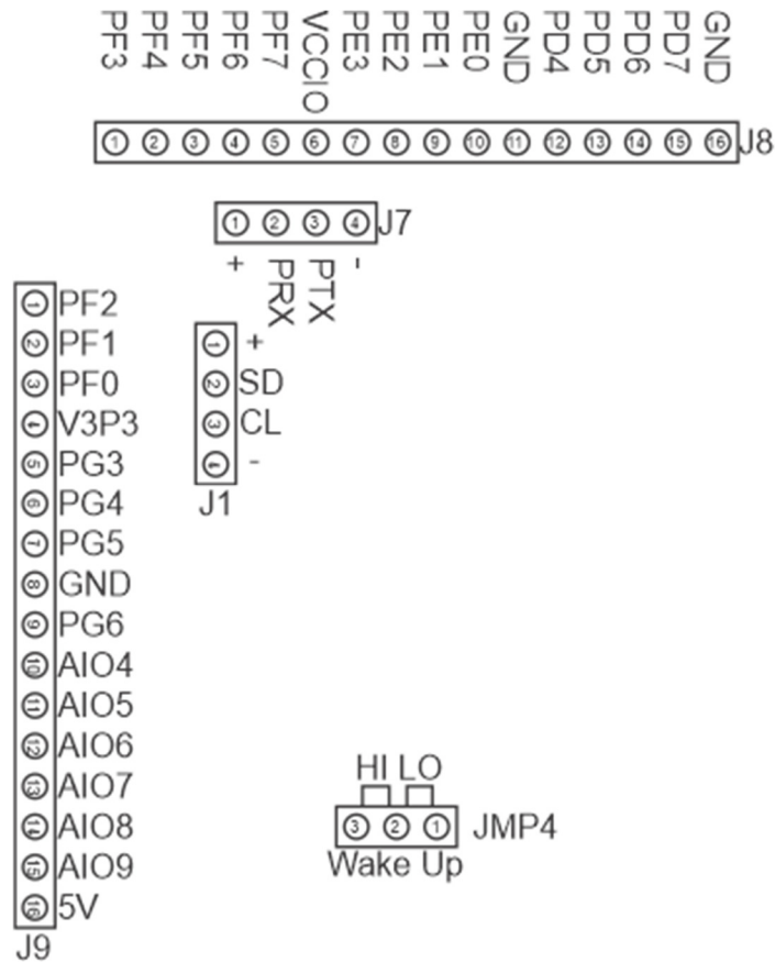
Figure 2 PAC5526EVK1 Headers and Test Stakes Pinout
