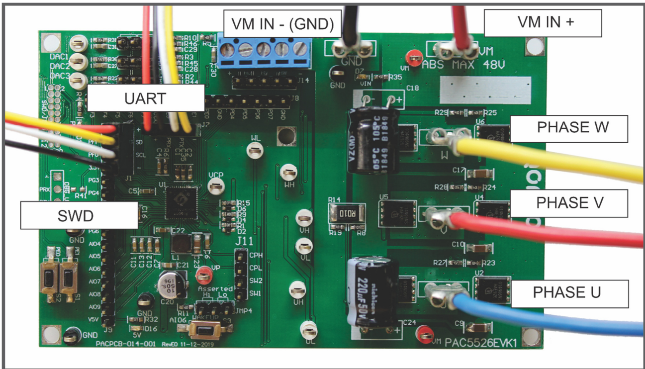
Figure 4: PAC5526EVK1 Evaluation Module Connections
