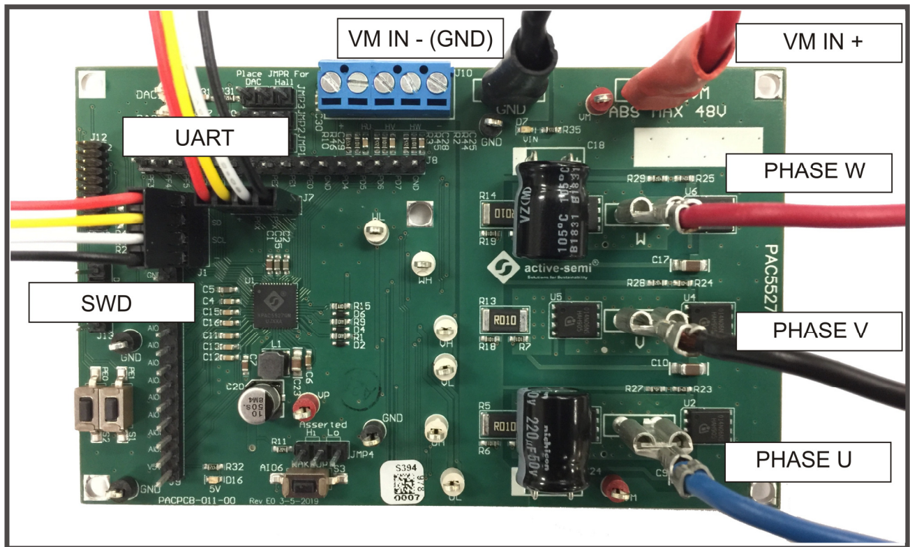
Figure 4: PAC5527EVK1 Evaluation Module Connections
