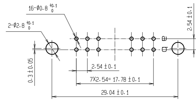
RECOMMENDED PC BOARD HOLE PATTERN(1:1)
