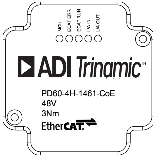
Figure 6: PD60-4H-1461-CoE LEDs
