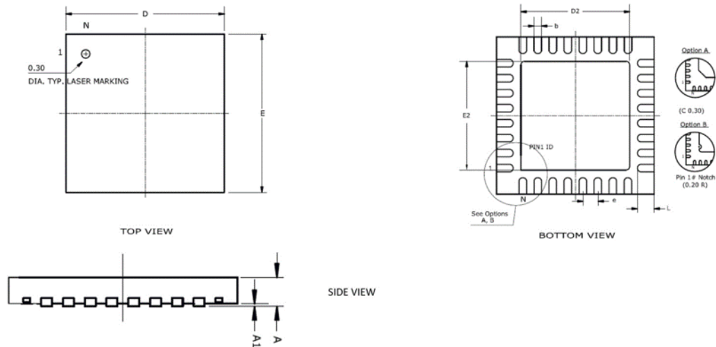
Figure 4-1. PD39210 Package Outline Drawing (32-Pin QFN 5 mm × 5 mm)
