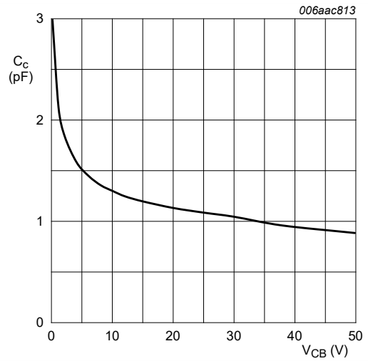
Fig. 15. PDTC123JQC-Q: Collector capacitance as a function of collector-base voltage; typical values
