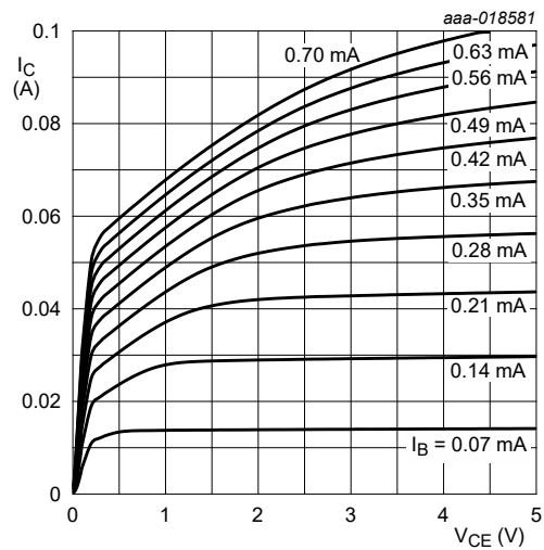
Fig. 17. PDTC143ZQC-Q: Collector current as a function of collector-emitter voltage; typical values
