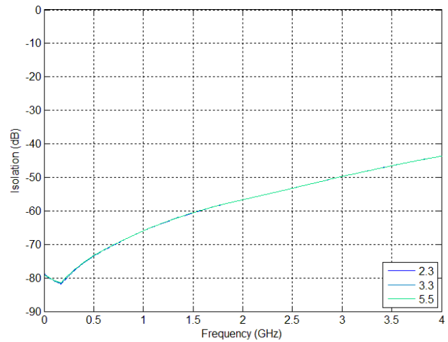
Figure 8. Isolation vs V_{DD} (RFC–RFX)
