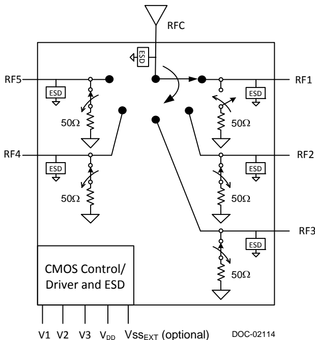
Figure 1. Functional Diagram
