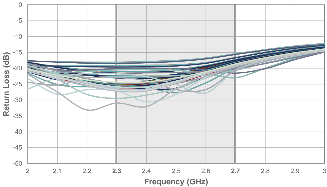
Figure 9 • Input Return Loss (All States)
