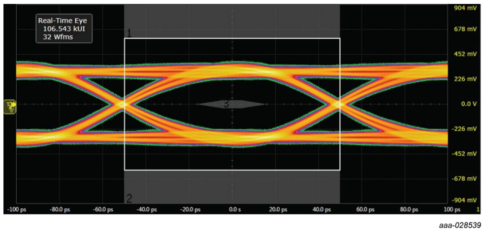
Fig. 5. USB 3.2 eye diagram 10 Gbps, test board without device; typical values
