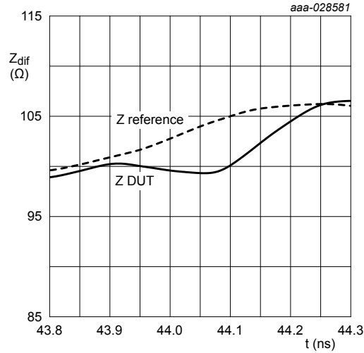
Fig. 3. Differential Time Domain Reflectometer (TDR) plot; typical values
