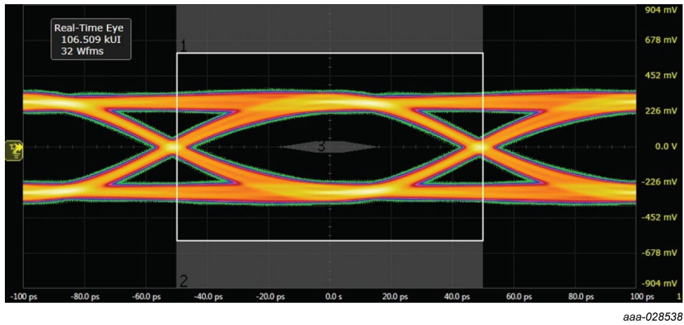
Fig. 4. USB 3.2 eye diagram 10 Gbps, test board with PCMFxUSB3B/C; typical values
