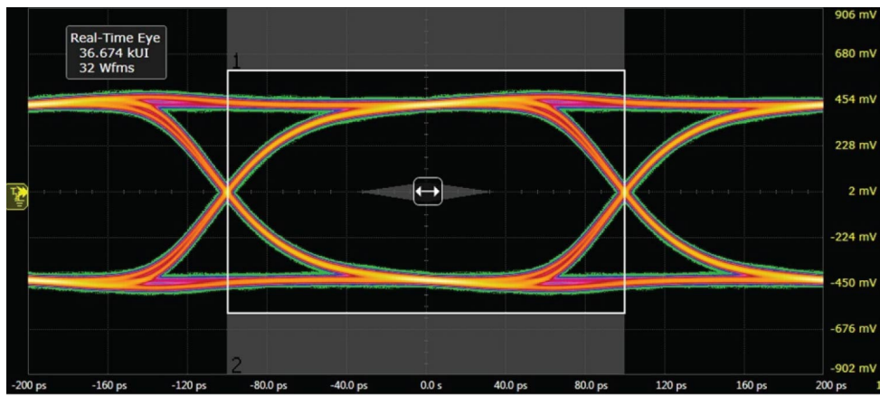
Fig. 6. USB 3.2 eye diagram 5 Gbps, test board with PCMFxUSB3B/C; typical values
