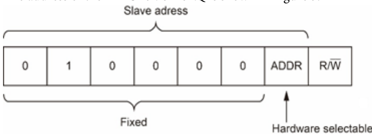
Figure 3. PI4IOE5V6416RQ Address
