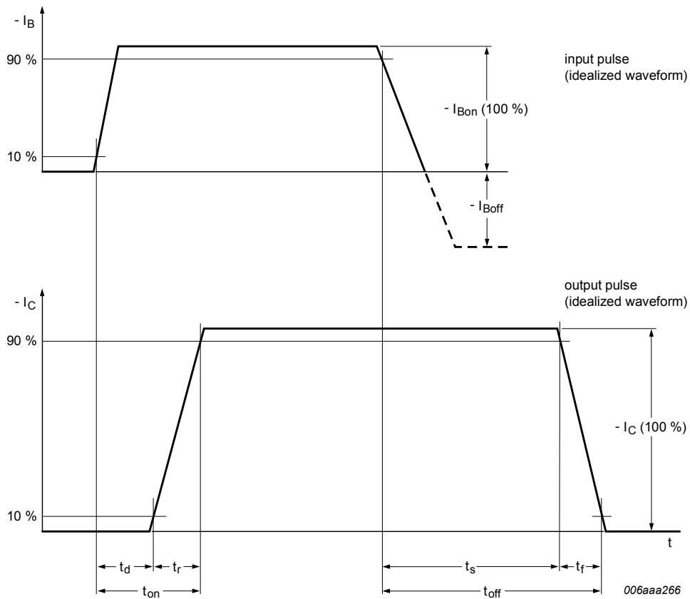
Fig. 10. Transistor switching time definition
