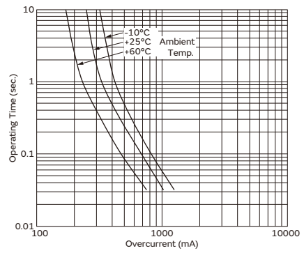
PRG21BC4R7MM1RA
