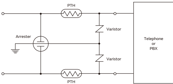
(5) Telecommunication Circuit
