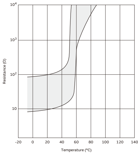
PTF_04BH471Q Type
