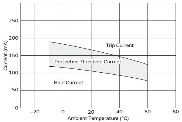
PTGL07AR560M9A51B0
