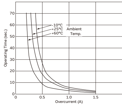
PTGL10BB120N0P52A0
