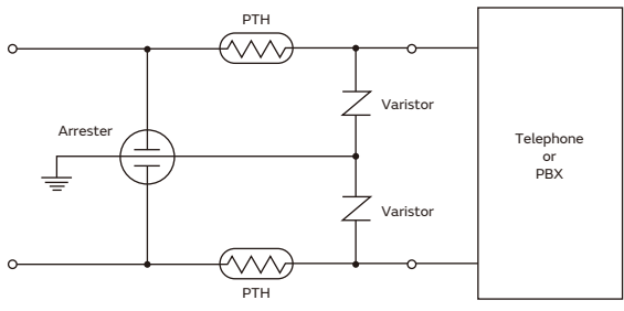
(5) Telecommunication Circuit
