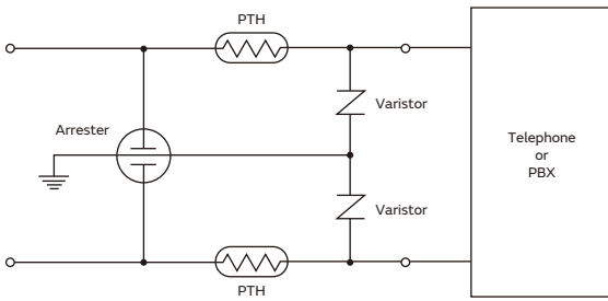
(5) Telecommunication Circuit
