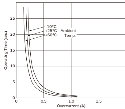
PTGL07AR560M9A51B0
