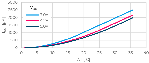
Figure 4. Output current for PRMT07-18305-** with 1/K_{TEC}=7\text{K/W}
