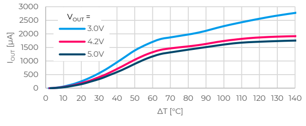
Figure 11. Output current for PRMT37-18305-**A with 1/K_{TEC}=37K/W
