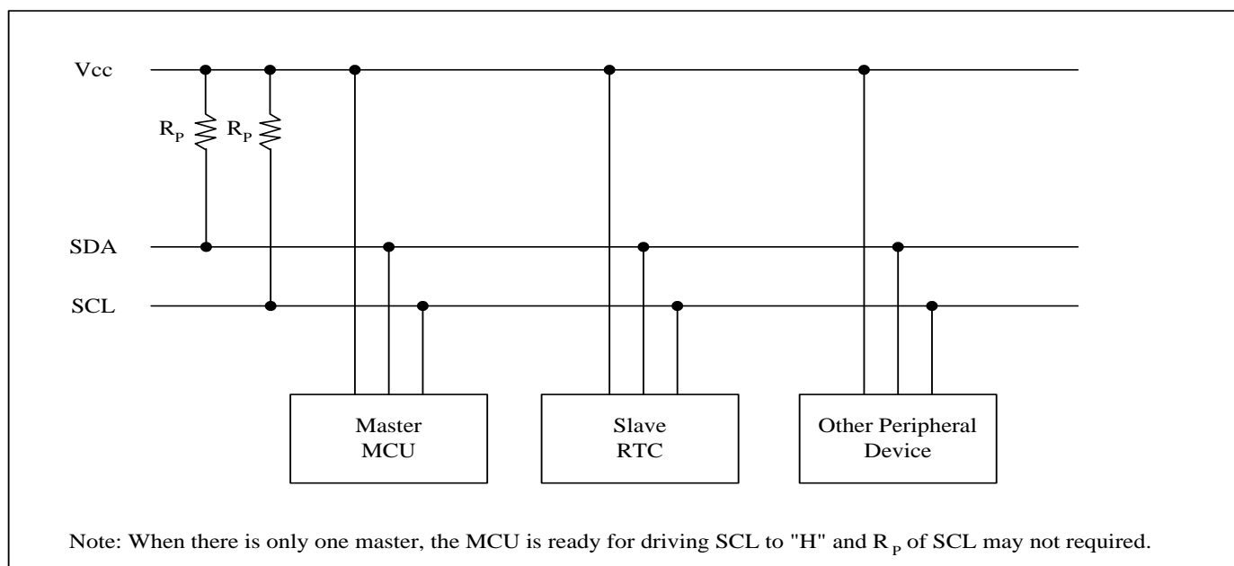
Fig.1 System configuration
