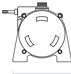
5.3" [135 mm]
