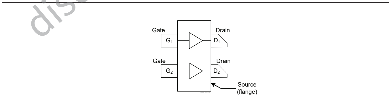
Lead connections for PTFB201402FC
