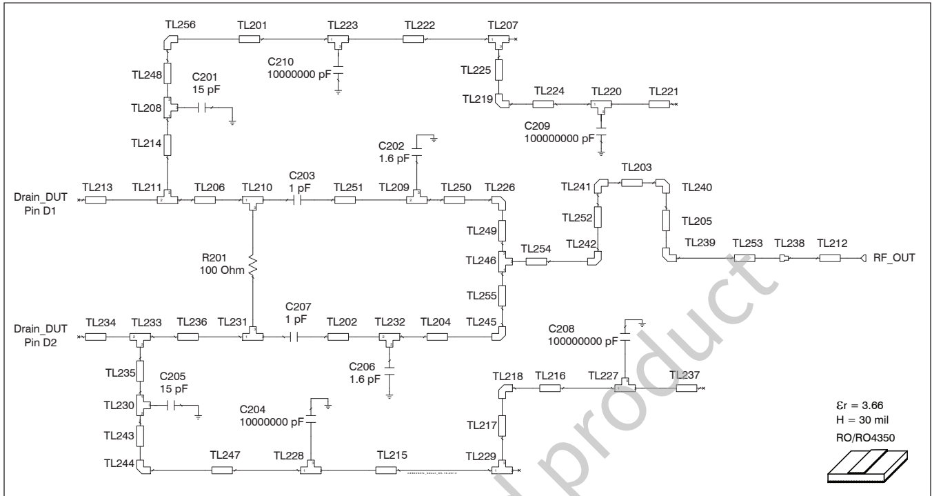
Reference circuit output schematic for f = 2680 \text{ MHz}
