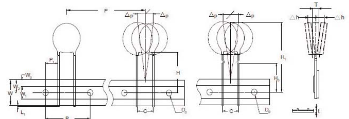
Figure 1 - PTR060V0010-PTR060V0185
