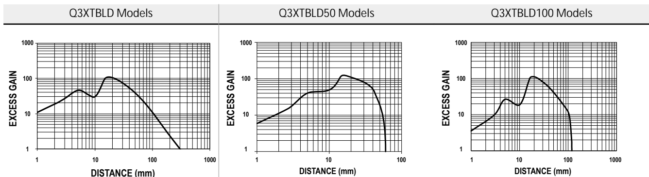
Figure 6. Excess Gain for Standard Sensitivity
