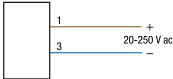
QD Emitters (4-pin Micro-Style)
