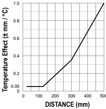
Figure 22. 500 mm Models
