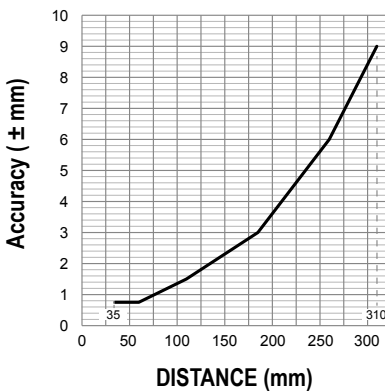
Figure 25. 310 mm Models
