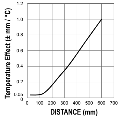
Figure 23. 600 mm Models
