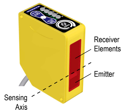
Figure 2. Sensing Axis
