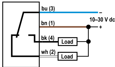
Figure 4. Complimentary NPN
