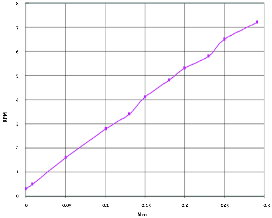
Figure 5.5: QBL4208-100-04-025 torque vs. current characteristics
