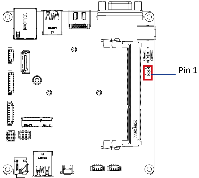
Back light brightness control connector
