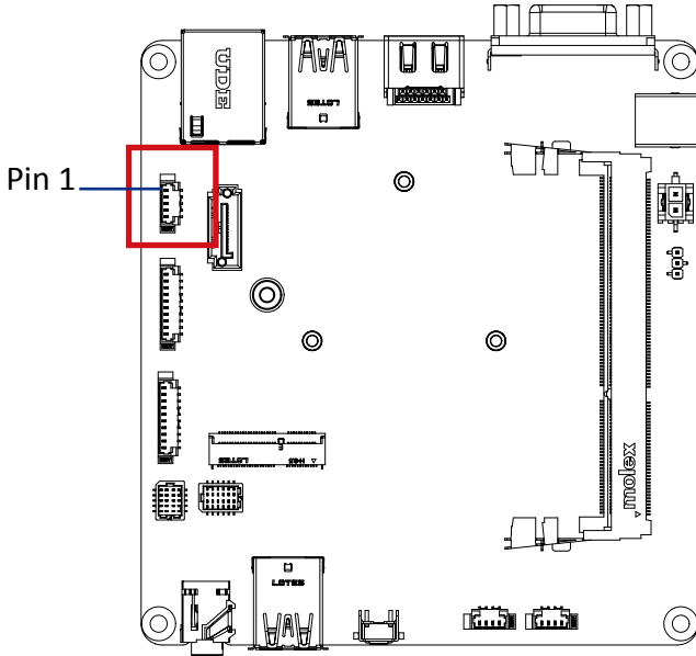
SATA 6Gb/s power connector
