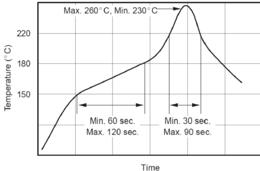
Figure 31: Reflow Profile of the WLCSP package
