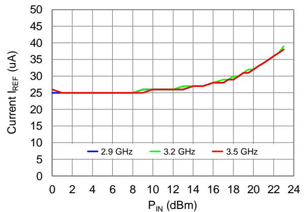
Current I_{REF} vs. P_{IN} vs. Frequency
