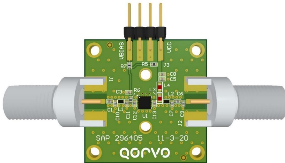
QPL1819 Evaluation Board
