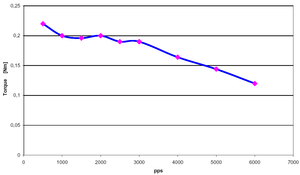
Figure 5.1: QSH4218-35-10-027 speed vs. torque characteristics
