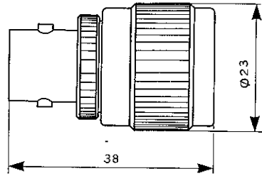
C MALE - HN FEMELLE
