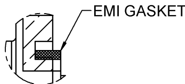
DETAIL B SCALE 6 : 1
