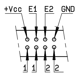
Solder pins
