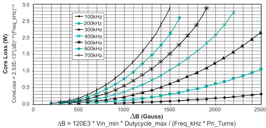
Core Loss vs. Flux Density
