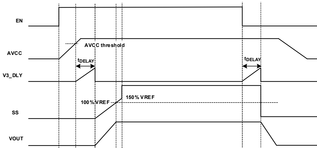
Figure 63. Delay Function
