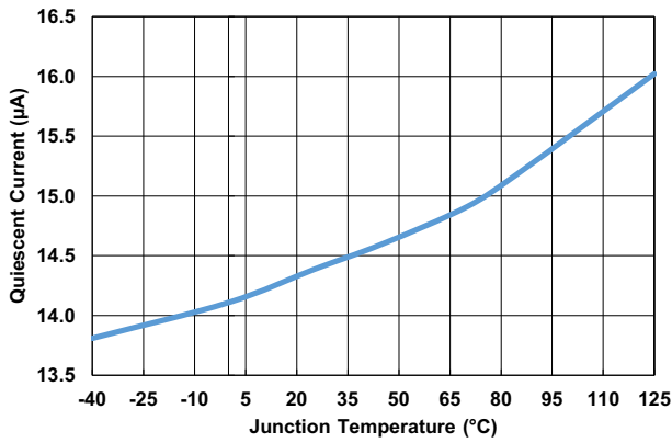
Figure 4. PVIN Quiescent Current vs Junction Temperature
