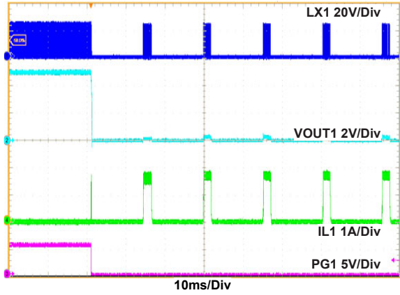
Figure 34. Overcurrent Protection Hiccup
