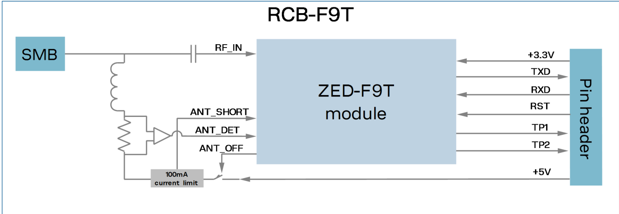
Figure 1: RCB-F9T-0 block diagram
