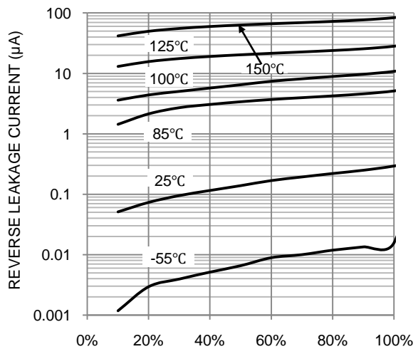
REVERSE LEAKAGE CURRENT ( \mu A ) V_R , PERCENTAGE RATED PEAK REVERSE VOLTAGE (%) Fig. 5 Typical Reverse Characteristics
