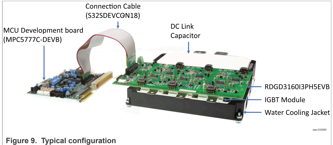
Figure 9. Typical configuration
