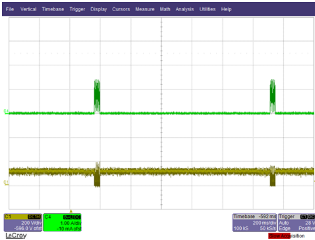
Figure 25 – 90 VAC, Full Load. Upper: I_{\text{OUTPUT}} , 1 A / div. Lower: V_{\text{DRAIN}} , 200 V, 200 ns / div.
