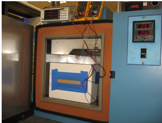
Figure 13 – Thermal Chamber Set-up Showing Box Used to Prevent Airflow Over UUT.
