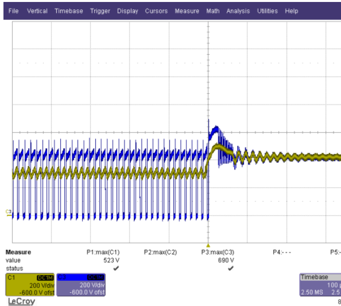
Figure 36 – 230 VAC / 60 Hz, 2 kV Differential Surge. Voltage Stress (U1): 690 V. Ch1: V_{BULK} , 200 V / div. Ch3: V_{SOURCE} , 200 V / div., 100 μs / div.
