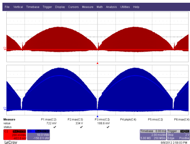
Figure 46 – 132 VAC, 60 Hz. Upper: I_{DRAIN} , 0.2 A / div. Lower: V_{DRAIN} , 50 V, 2 ms / div.
