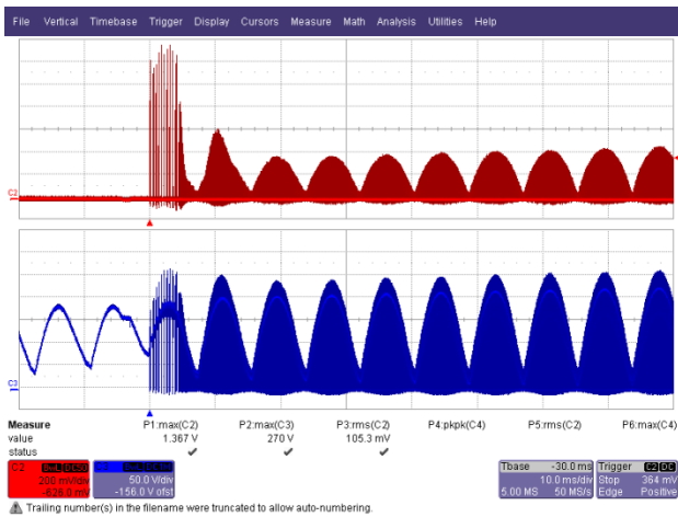
Figure 50 – 132 VAC, 60 Hz Start-up. Upper: I_{DRAIN} , 200 mA / div. Lower: V_{DRAIN} , 50 V, 5 ms / div.
